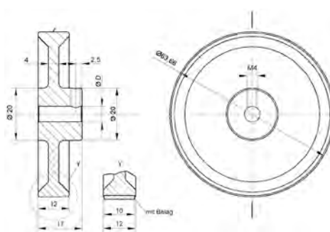
Measuring wheel 200 mm circumference
